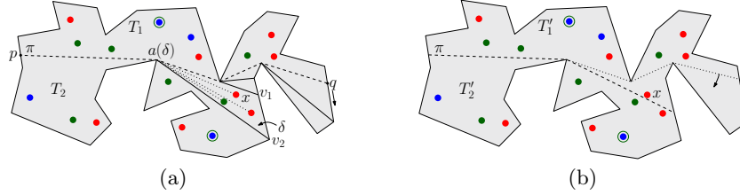
Fig. 10. Removing a point x from T_2 and add it to T_1 by adjusting \pi . (a) A sweep-path which is anchored at p and sweeps the polygon, in clockwise order, from q . (b) The adjusted geodesic (in dashed lines).
