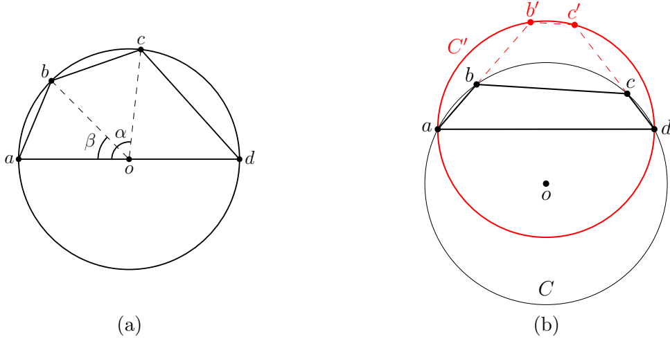
Figure 5: (a) Proof of Lemma 5 and Lemma 6. (b) Proof of Lemma 6.
