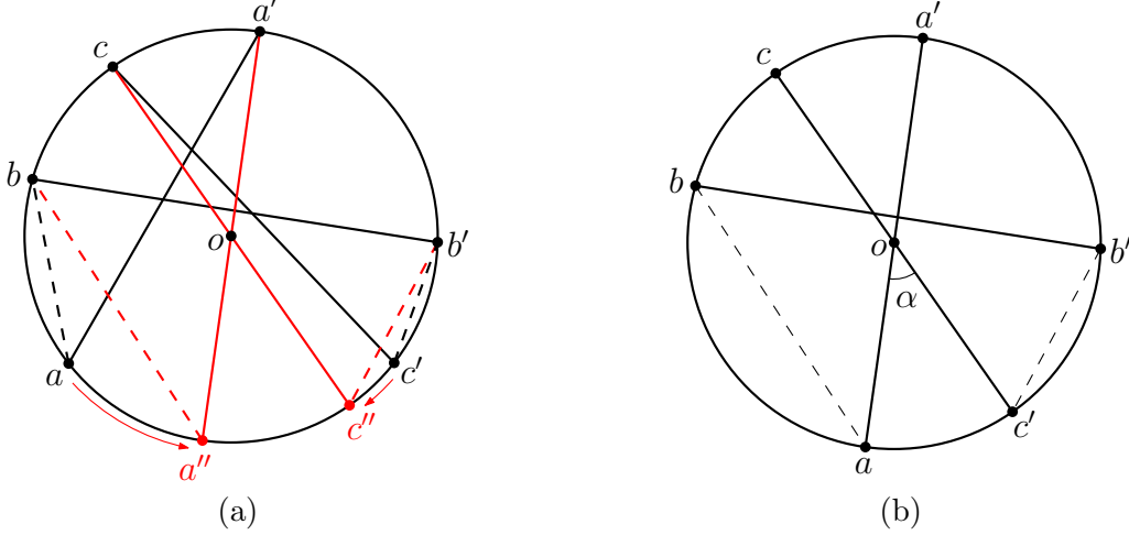
Figure 7: Proof of case (ii) in Theorem 1.
