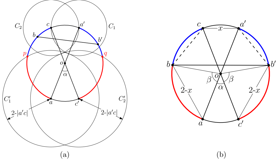
Figure 8: Proof of case (ii) in Theorem 1.
