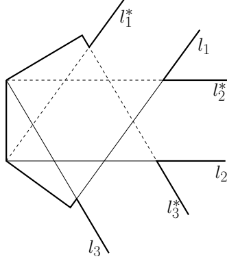
Figure 5: Result of the right envelope algorithm (shown in fat)
