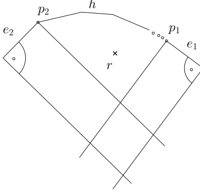
Figure 4: Location of a point r in a bounded region.
