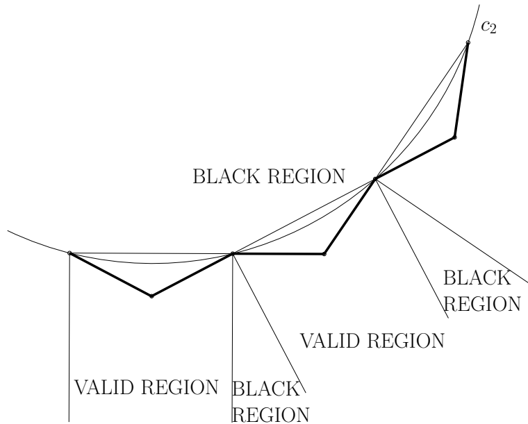
Figure 8: Polygonal chain
