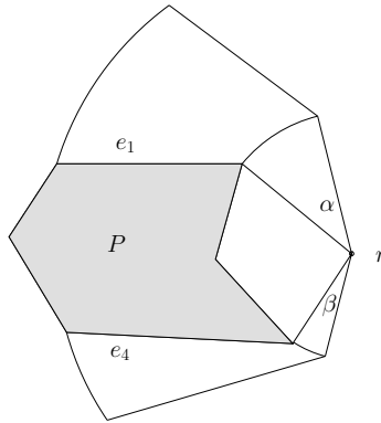
Figure 1: The edges e_1 and e_4 are removable in cw orientation with angle \alpha and ccw orientation with angle \beta with respect to r respectively.
