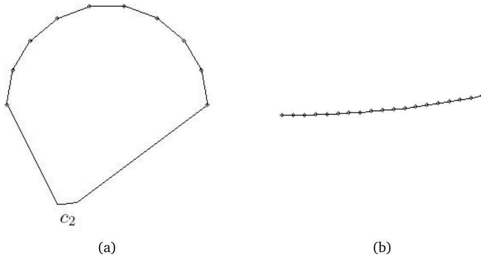
Figure 9: Example with s = 10 . (a) shows the polygon, (b) shows an enlargement of the polygonal chain c_2 .
