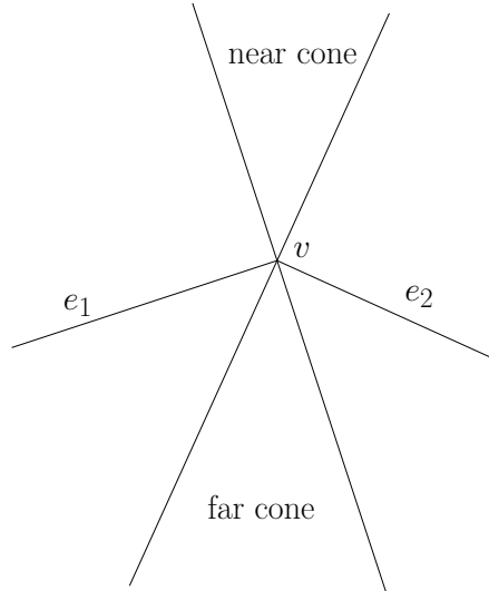
Figure 6: The near cone and the far cone of v .
