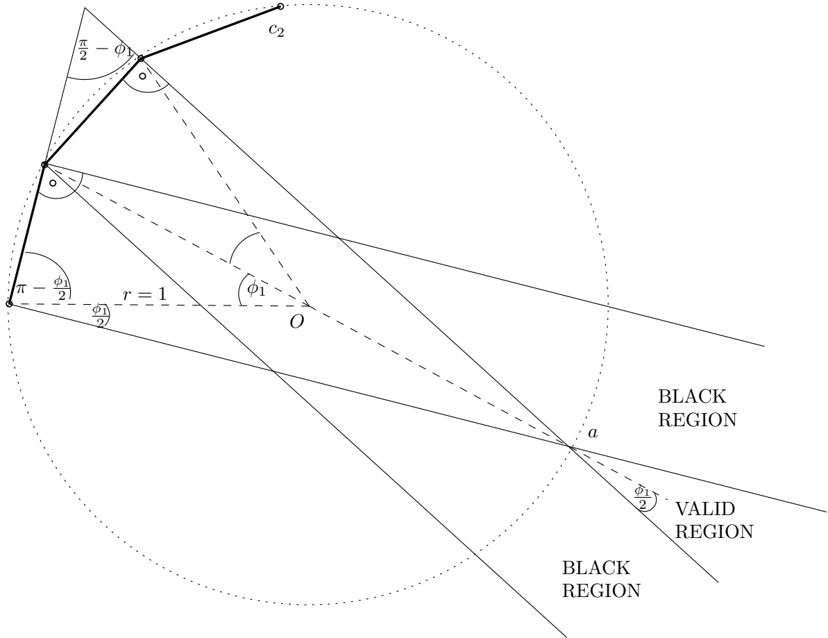
Figure 7: Approximation of half circle
