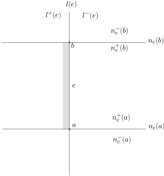
Figure 2: The half planes associated with an edge e .
