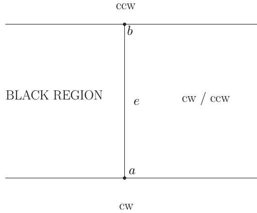
Figure 3: An edge splits the plane into regions of different valid orientations for cast removal
