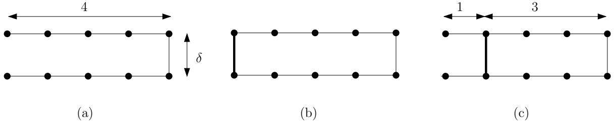
Figure 2: (a) The input graph G . (b) The bottleneck solution compared to (c) the optimal solution.
