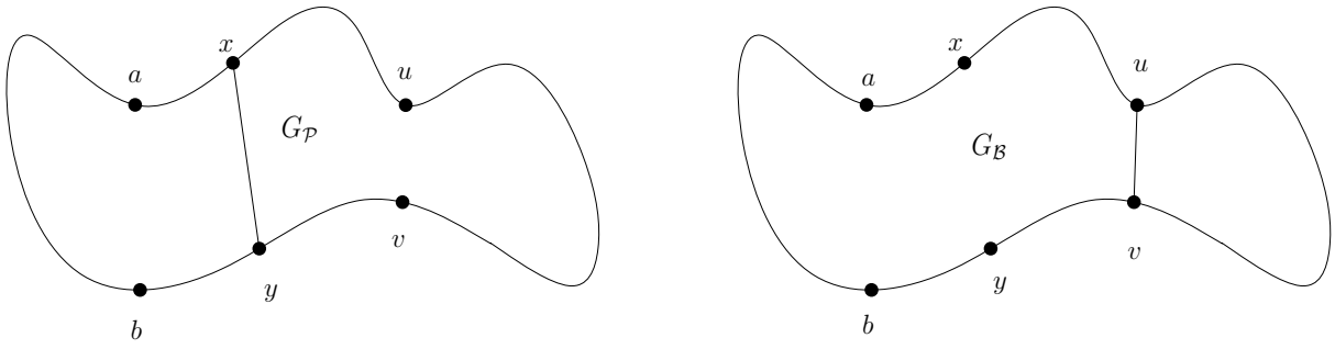
Figure 1: (x, y) is the optimal edge added to G and (u, v) is a bottleneck edge.
