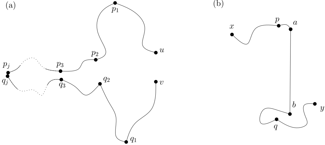
Figure 3: (a) Illustrating the proof of Lemma 5. (b) Illustrating the proof of Lemma 6.
