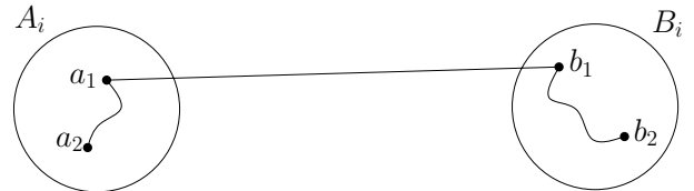
Figure 4: Illustrating Lemma 8.
