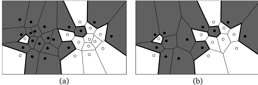
Figure 1: The Voronoi diagram (a) before Voronoi condensing and (b) after Voronoi condensing. Note that the decision boundary (in bold) is unaffected by Voronoi condensing. Note: In this figure, and all other figures, red points are denoted by white circles and blue points are denoted by black disks.
