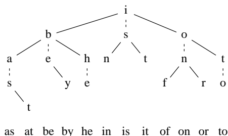
Figure 2. A ternary search tree for 12 two-letter words
