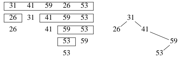
Figure 1. Quicksort and a binary search tree
